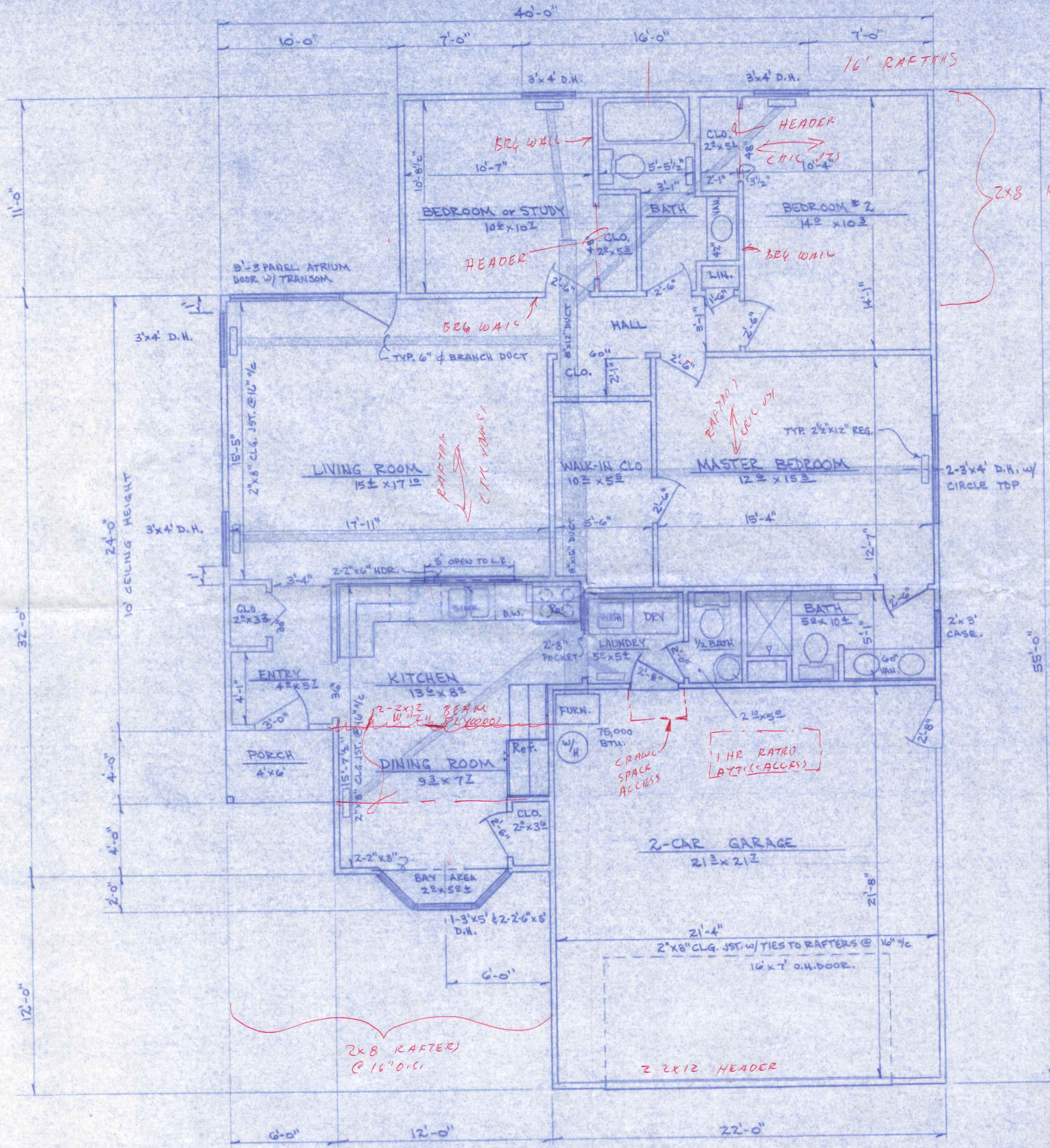
FLOOR PLAN w/HEATING LAYOUT 1/4" = 1'-0"
